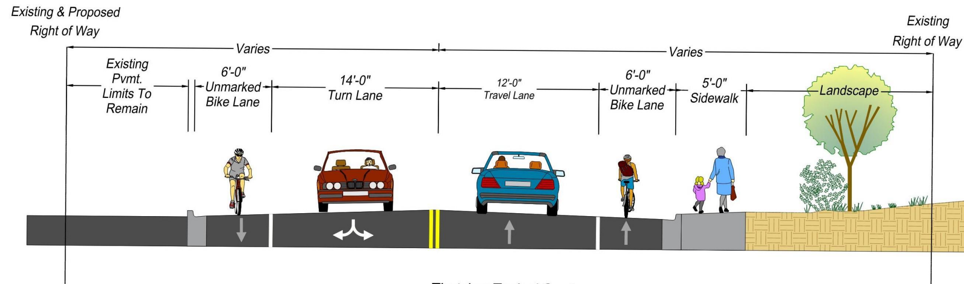
Thatcher Typical Section At Gales Creek Intersection
