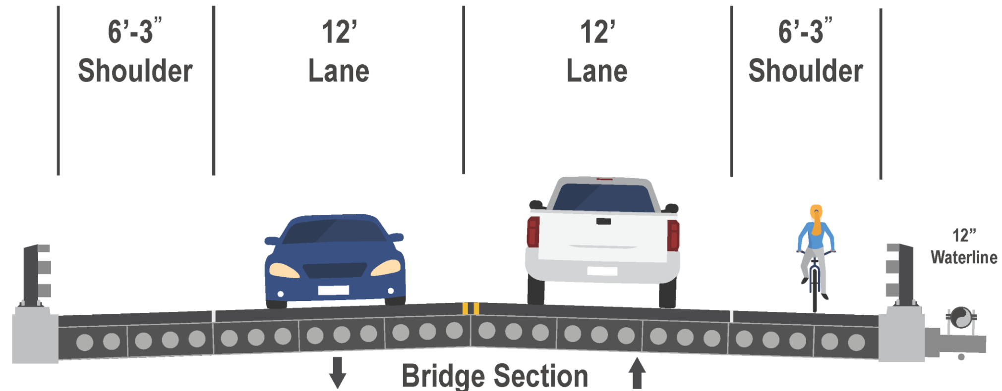
Martin Road Typical Section
