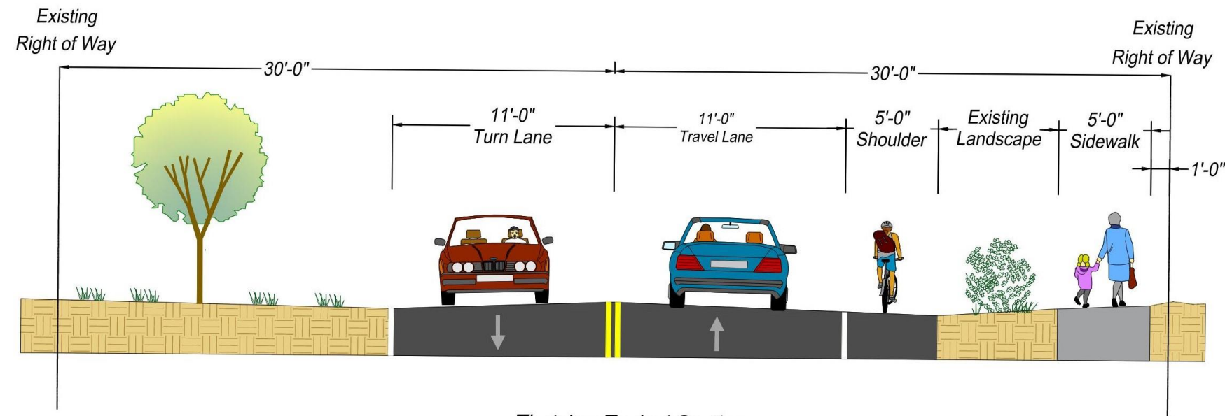
Thatcher Typical Section
