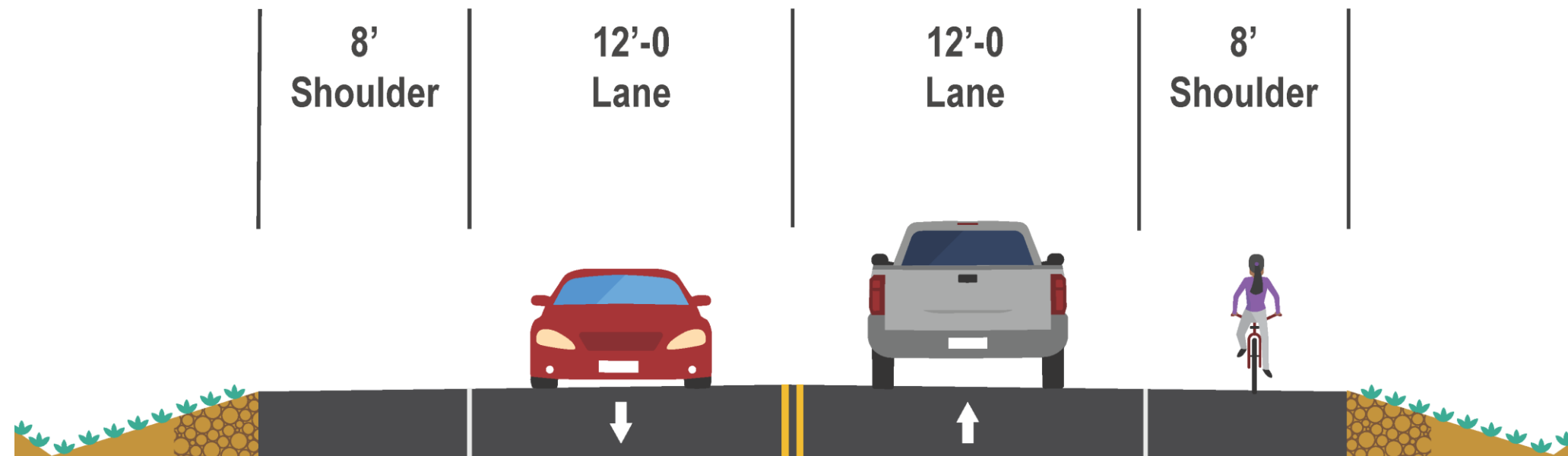
Martin Road Typical Section
