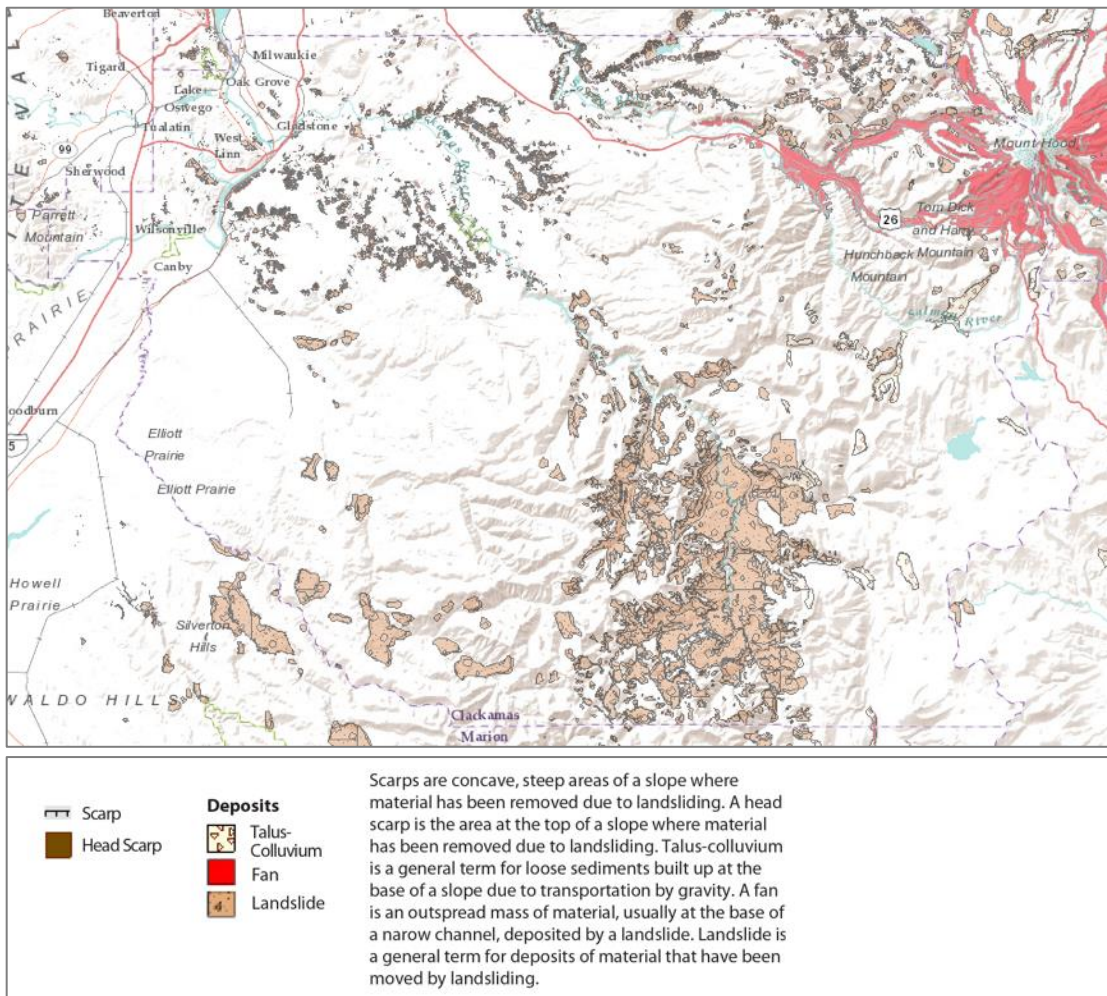
Figure 2-15 Landslide Inventory
