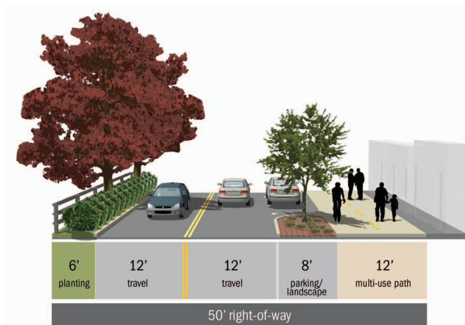
Figure A-4. Conceptual Cross-Section for Main Street – Milport Road to Beta Street with additional right-of-way and multi-use
