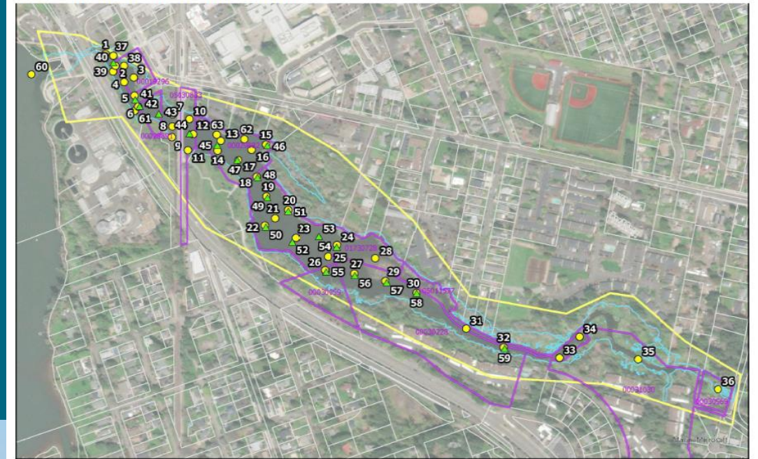
Phase 2 - Proposed Boring Locations
